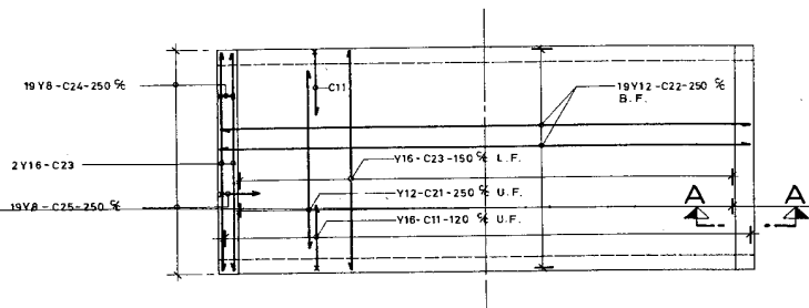
PLAN OF TOP SLAB.
