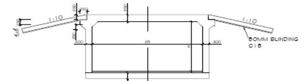
SECTION C 1:75
