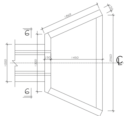
PART PLAN SCALE 1:25
