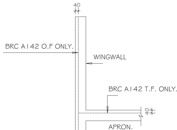
SECTION 7 - 7.
