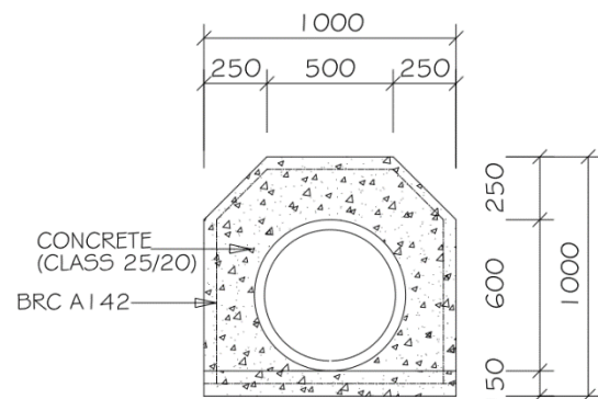
SECTION 6 - 6. SCALE 1:25
