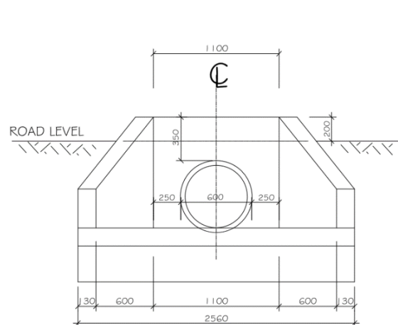
ELEVATION SCALE 1:25
