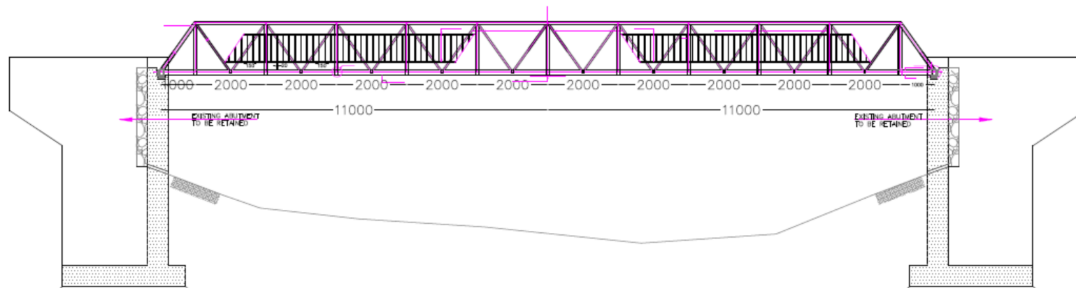
LHS FOOTBRIDGE ELEVATION
