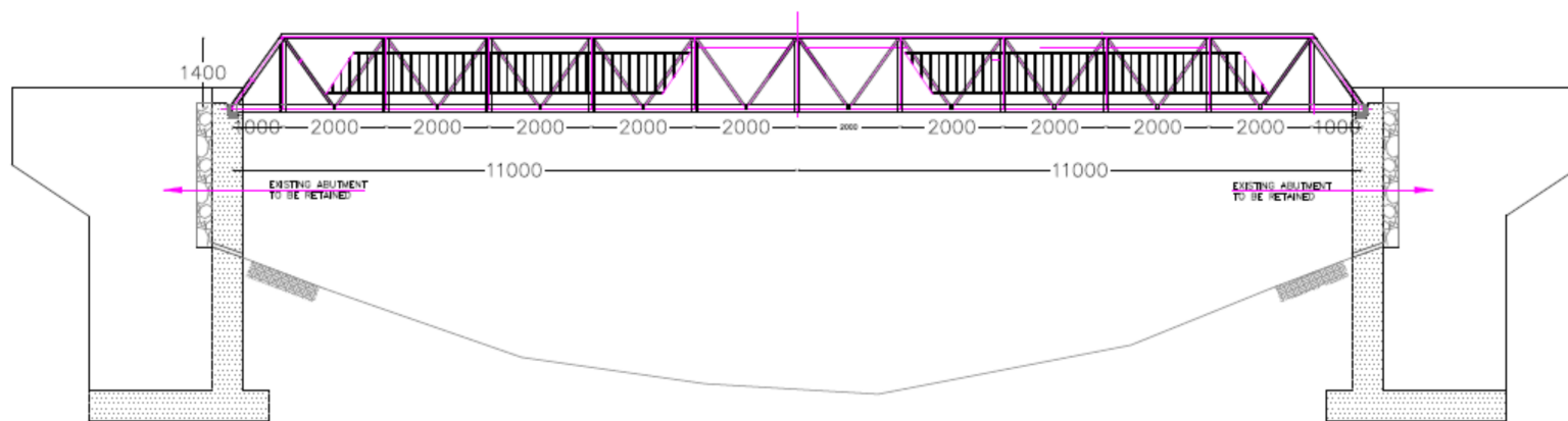
RHS FOOTBRIDGE ELEVATION
