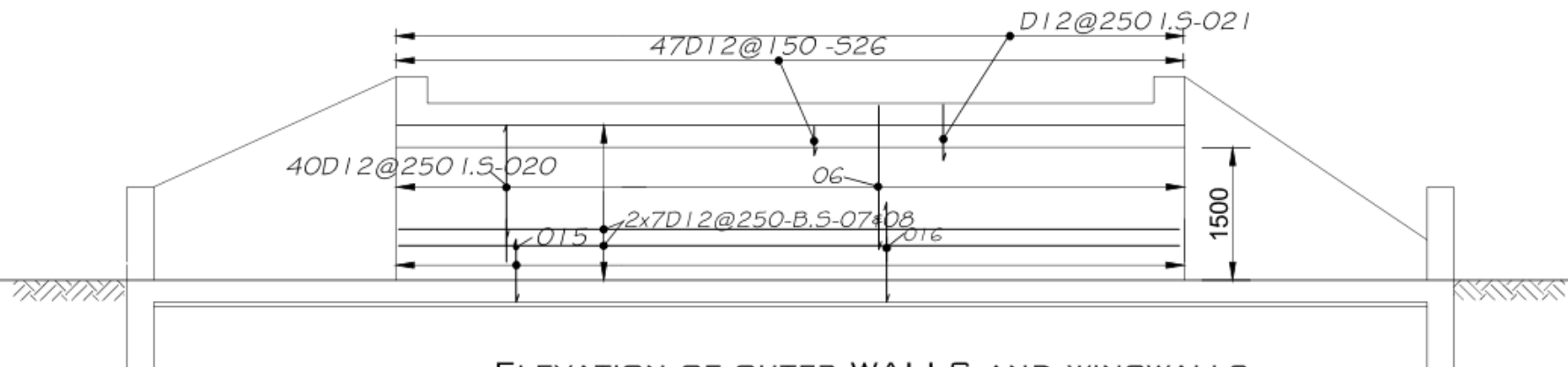
ELEVATION OF OUTER WALLS AND WINGWALLS
