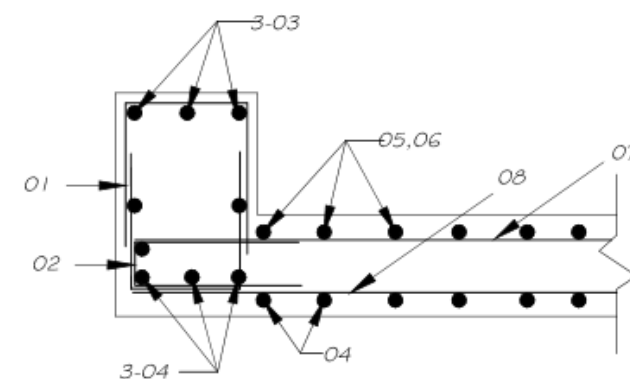
APPROACH SLAB
