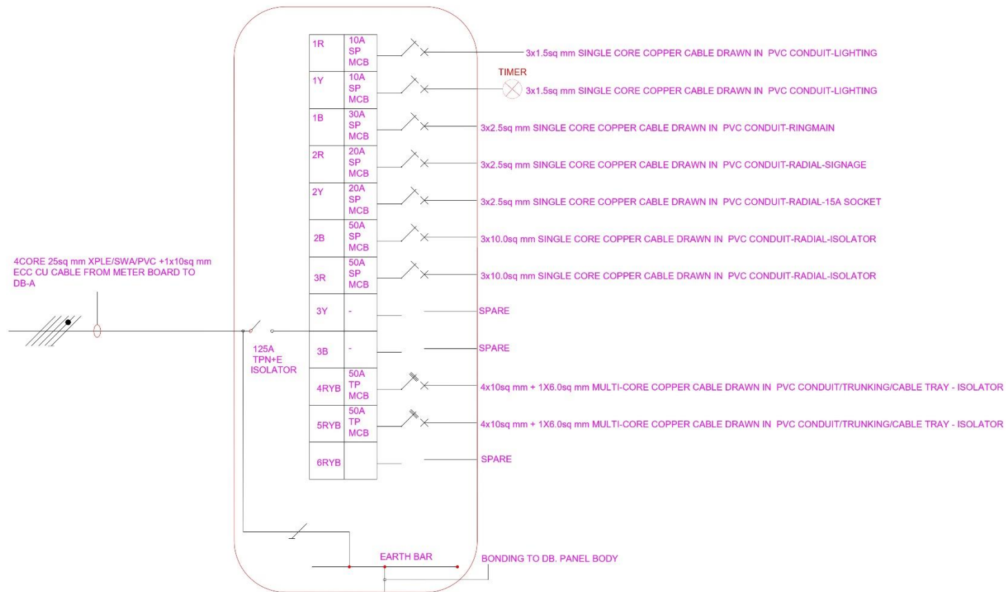
6 WAYS 125A TPN FLUSH MOUNTED DISTRIBUTION BOARD COMPLETE WITH FRONT LATCHED COVER AS DB-A
