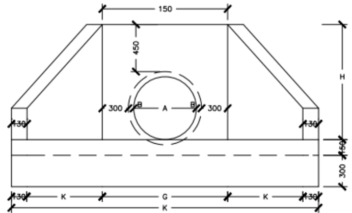
FRONT ELEVATION-SINGLE CELL
