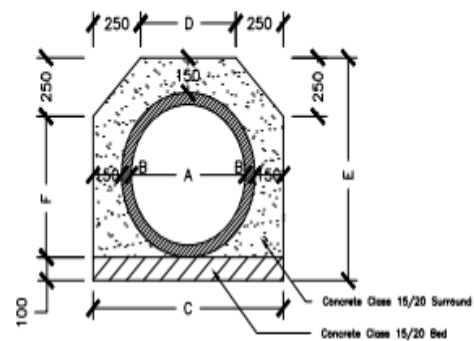
TYPICAL CONCRETE BED AND SURROUND-SINGLE CELL
