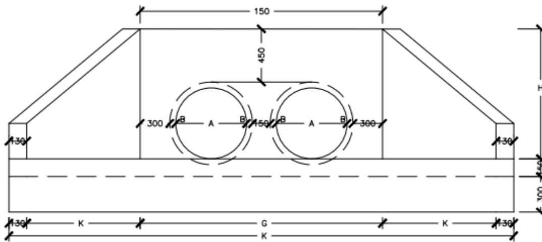
FRONT ELEVATION—MULTIPLE CELL
