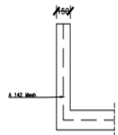
TYPICAL CONCRETE BED AND SURROUND-SINGLE CELL
