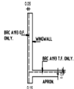
SECTION C - C.
