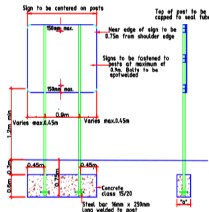
SIGN AND FOUNDATION DETAILS NOT TO SCALE
