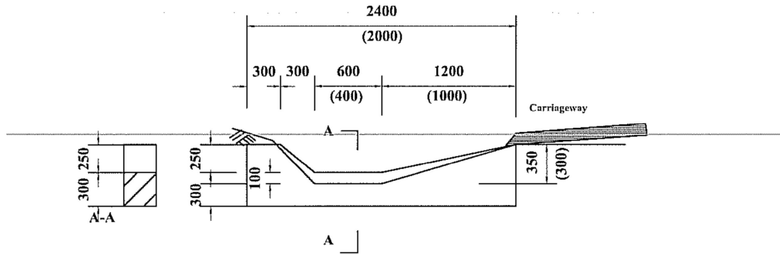
SECTION OF CONCRETE SCOUR CHECK
