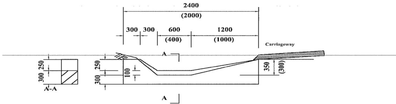
SECTION OF CONCRETE SCOUR CHECK
