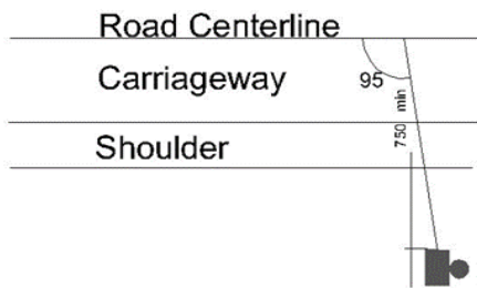
TYPICAL SIGN LOCATION PLAN
