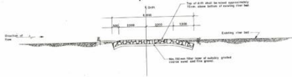
Section A Scale 1:50
