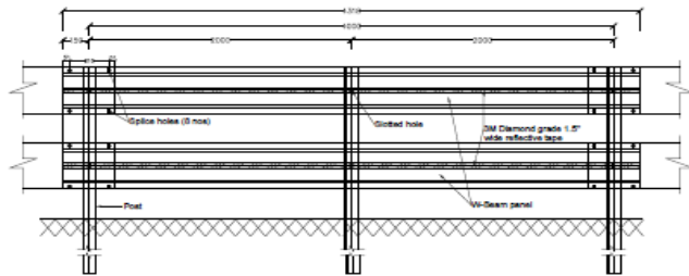
W-Beam panel section
