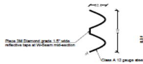
W-Beam panel section
