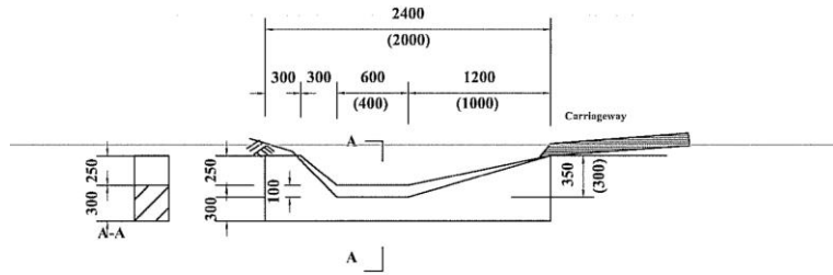
SECTION OF CONCRETE SCOUR CHECK
