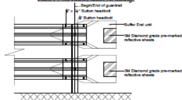
Buffer End Connection Detailing
