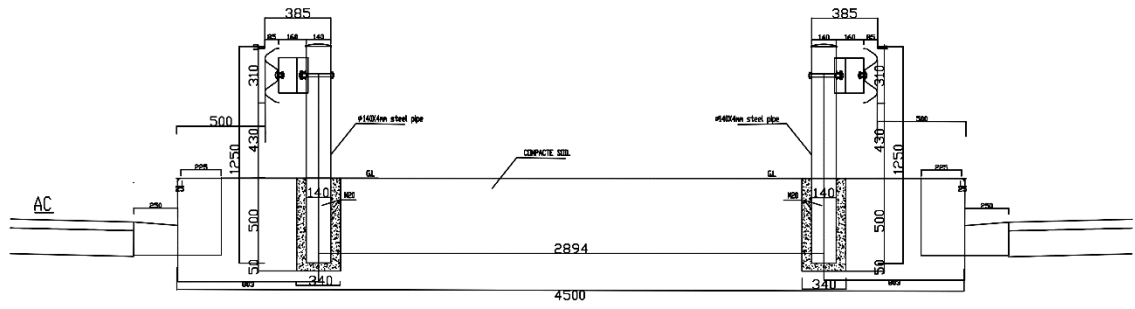
GUARDRAILS ELEVATION
