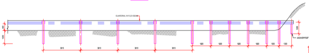
ALTERNATIVE GUARDRAIL END TREATMENT SCALE:-1:100
