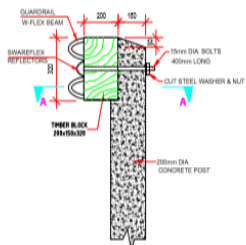
ARRANGEMENT AT THE POST SCALE:-1:10
