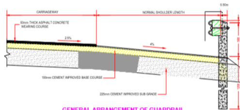
GENERAL ARRANGEMENT OF GUARDRAIL SCALE:-1:10
