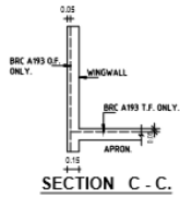
SECTION C - C.
