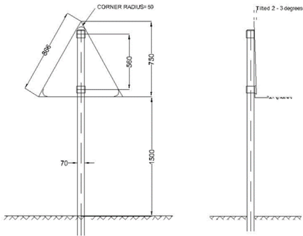
WARNING SIGN
