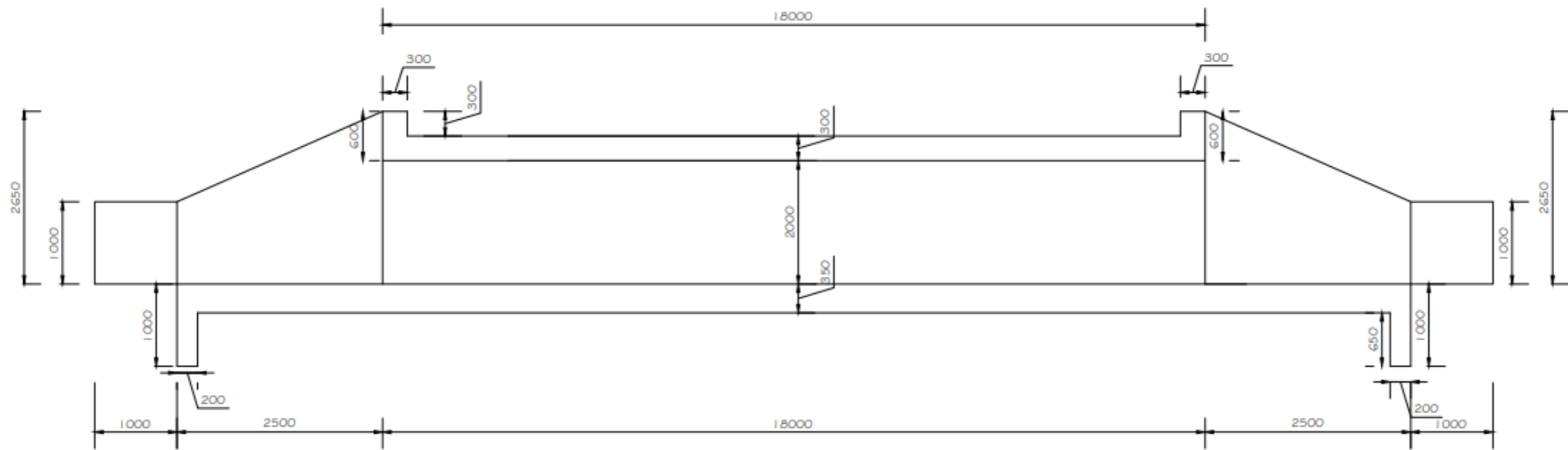
SECTION C-C
