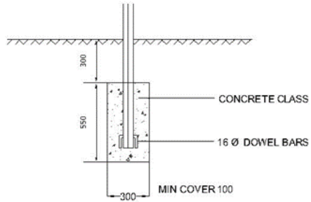
FOUNDATION DETAILS
