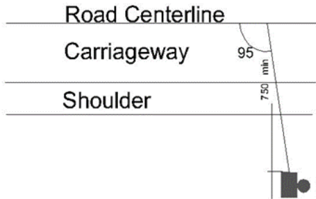
TYPICAL SIGN LOCATION PLAN
