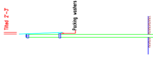
TYPICAL SIDE ELEVATION
