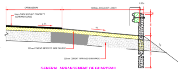
GENERAL ARRANGEMENT OF GUARDRAIL SCALE:- 1:10
