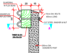
ARRANGEMENT AT THE POST SCALE:- 1:10
