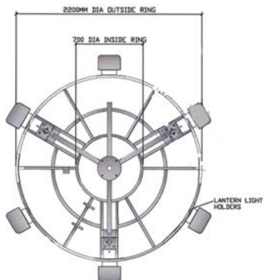
PLAN VIEW OF ENLARGED CARRIAGE RINGS + DETAILS ( 9 nos of light)
