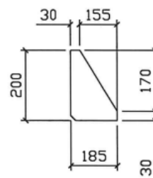
12NOS BASE PLATE STIFFENER-SF1
