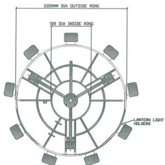
PLAN VIEW OF ENLARGED CARRIAGE RINGS + DETAILS ( 9 nos of light)
