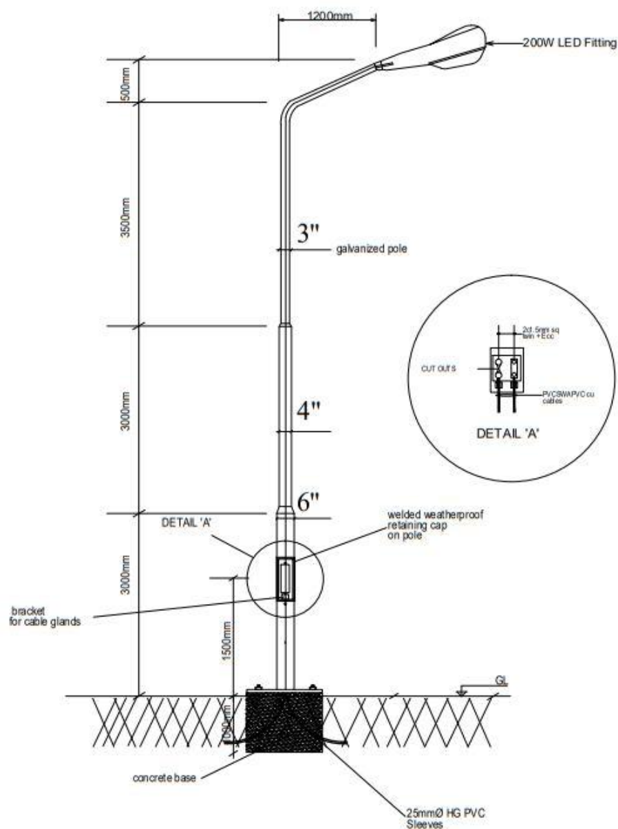
CROSS SECTIONAL DRAWING - SINGLE ARM POLE
