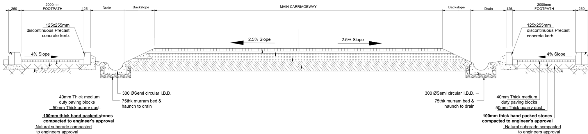
TYPICAL SECTION THROUGH THE ROAD & 2.0M WALKWAY SCALE 1:25
