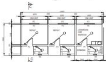
JUNIOR TECHNICIANS HOUSES (BLOCK OF 3 HOUSES)-HOUSE TYPE V
